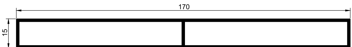
P.31 Tube Rectangular 170*15*1.45mm
