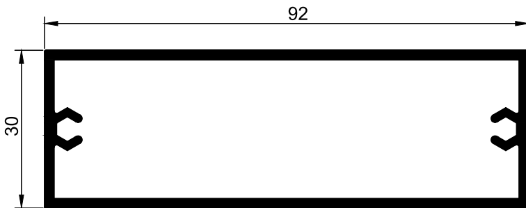
ST.73 Tube Rectangular 92*30*1.4mm
