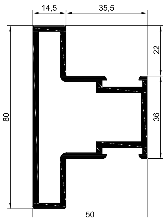
PT.03 Travessa
