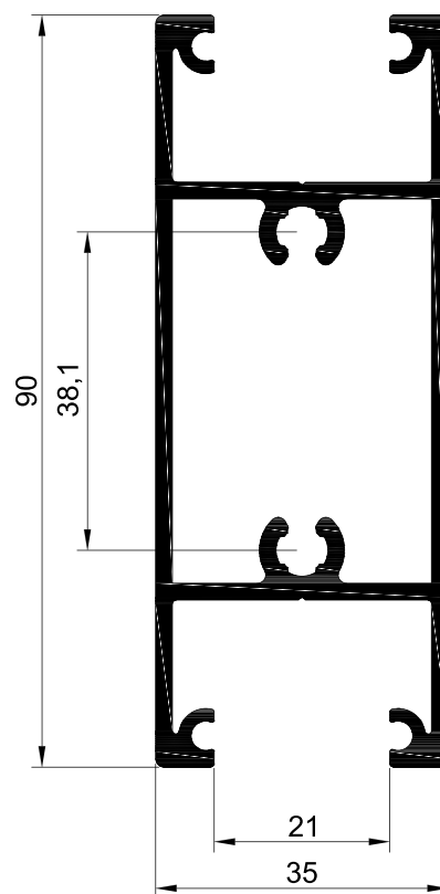
PT.236 Travessa Central
