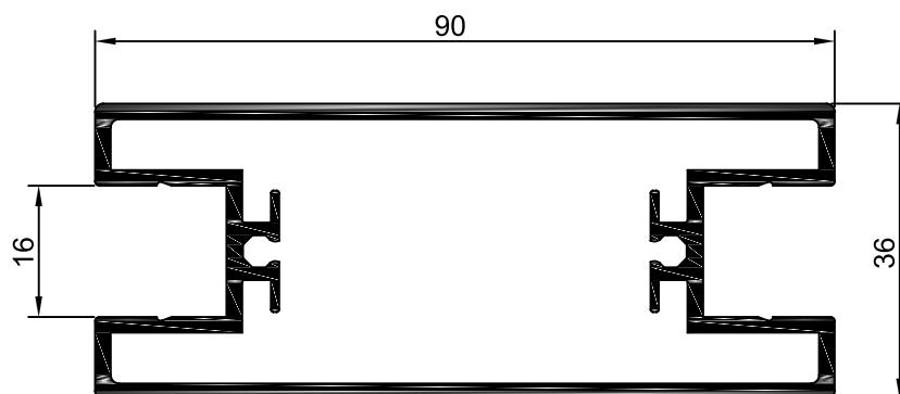
PT.107 Travessa Central
