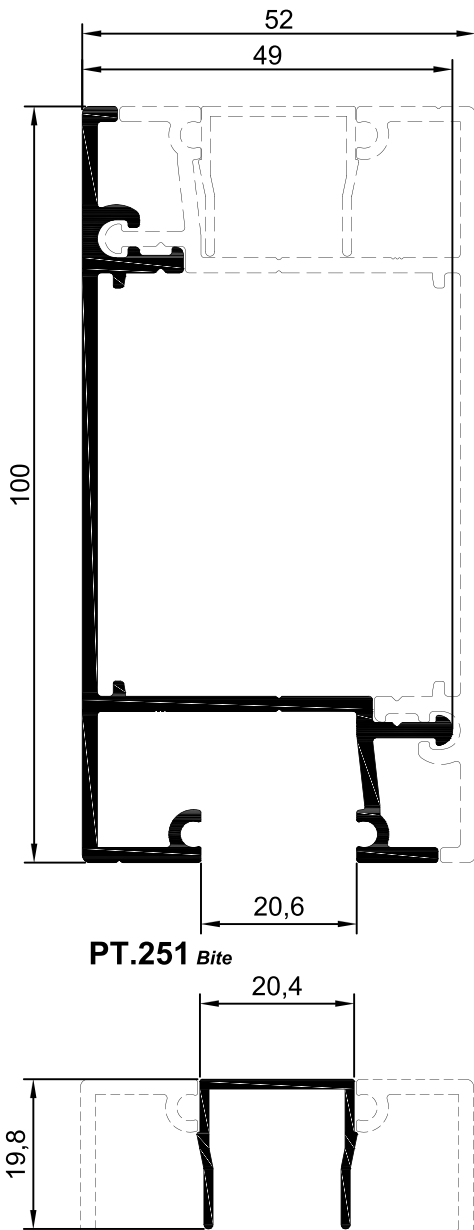
PT.261 Prumo Vertical ( Grades )
