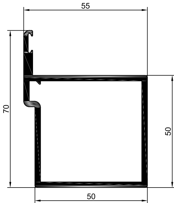
PT.03 Travessa
