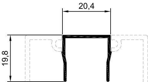
PT.251 Bite
